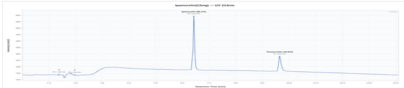
Tesamorelin / Ipamorelin 13mg - 0720340-CP012606263513L: UV Chromatogram
